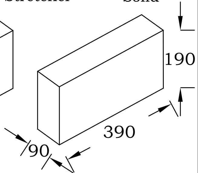
Solid
