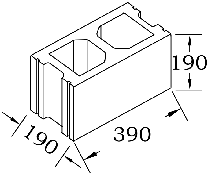
Regular Stretcher
