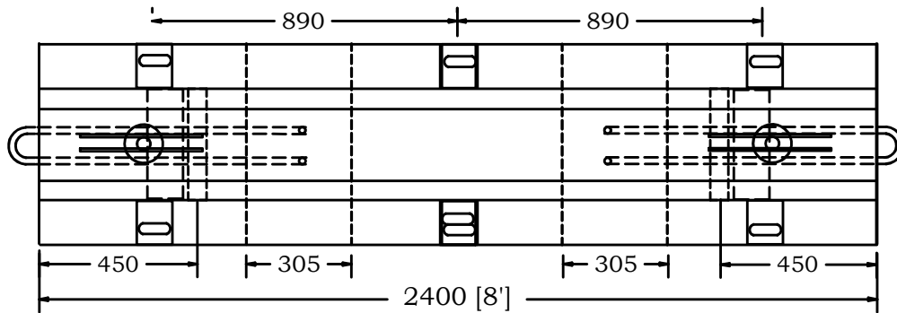
PLAN VIEW
