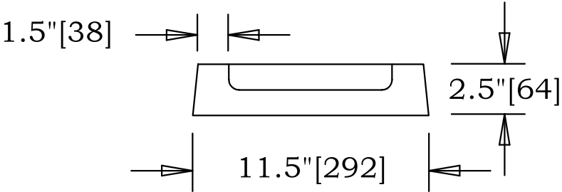
End View
